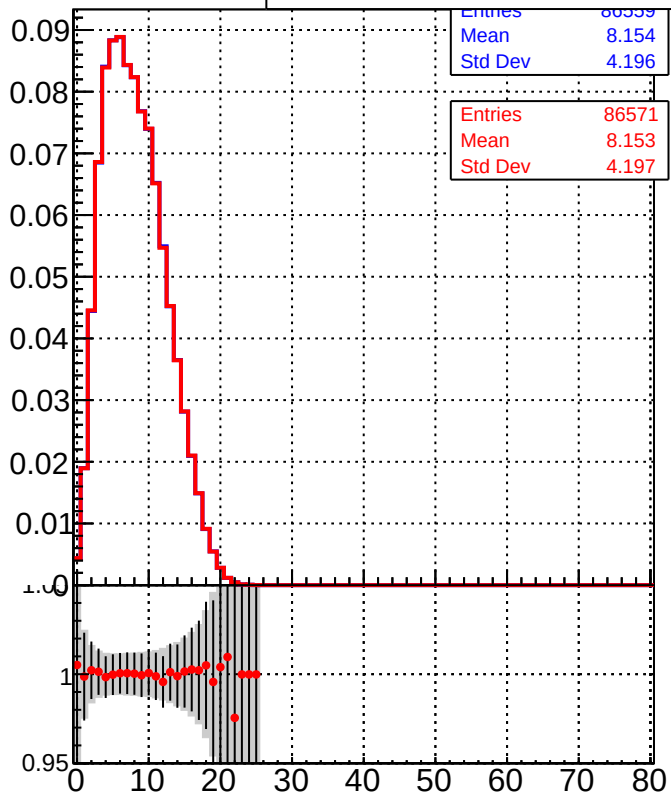
Legend: DQM_TT_mkFit-DQM_lowptq_orig (gray bars), DQM_TT_mkFit-DQM_lowptq_modi2 (red line)
