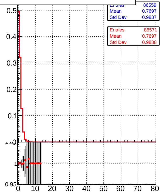
Legend: DQM_TT_mkFit-DQM_lowptq_orig (gray bars), DQM_TT_mkFit-DQM_lowptq_modi2 (red line)
