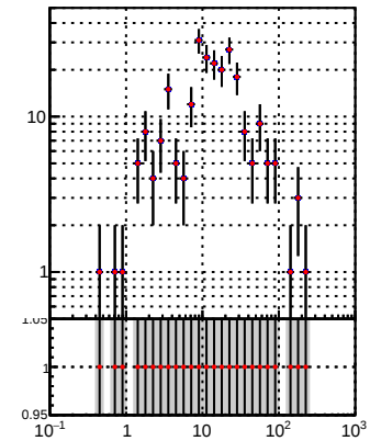
—●— DQM_TT_mkFit-DQM_lowptq_orig —●— DQM_TT_mkFit-DQM_lowptq_modi2
