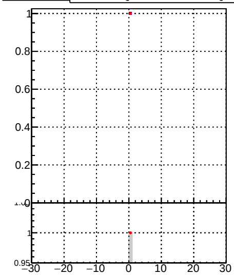
Fake rate vs vertpos Legend: DQM_TT_mkFit-DQM_lowptq_orig DQM_TT_mkFit-DQM_lowptq_modi2
