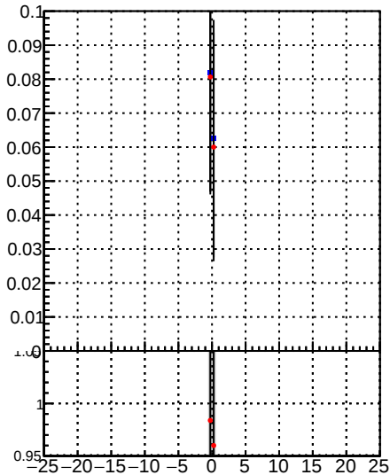
Fake rate vs d —•— DQM_TT_mkFit-DQM_lowptq_orig —•— DQM_TT_mkFit-DQM_lowptq_mod12
