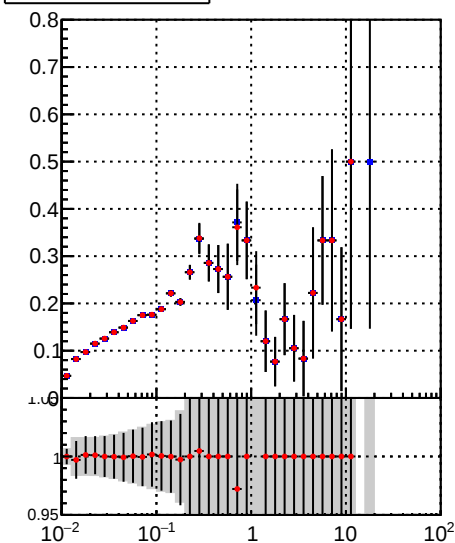
—•— DQM_TT_mkFit-DQM_lowptq_orig —•— DQM_TT_mkFit-DQM_lowptq_modi2
