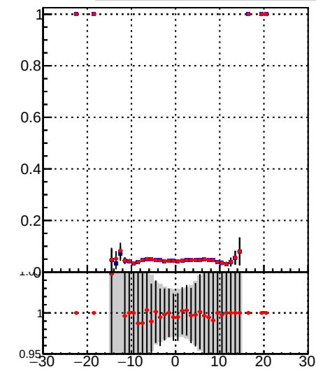
—•— DQM_TT_mkFit-DQM_lowptq_orig —•— DQM_TT_mkFit-DQM_lowptq_modi2
