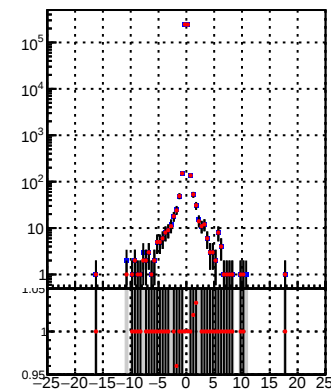
—•— DQM_TT_mkFit-DQM_lowptq_orig —•— DQM_TT_mkFit-DQM_lowptq_modi2
