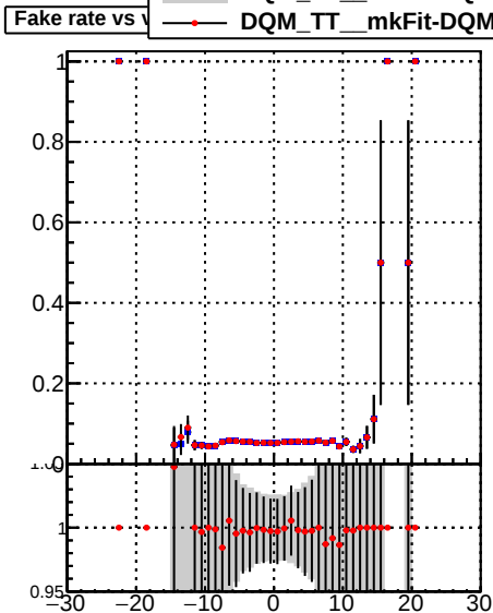
—■— DQM_TT_mkFit-DQM_lowptq_orig —●— DQM_TT_mkFit-DQM_lowptq_modi2
