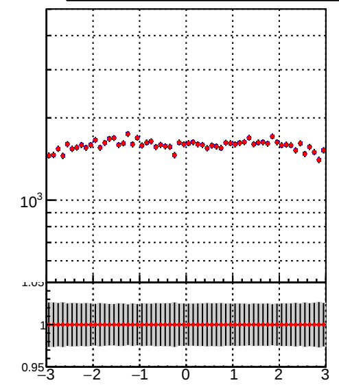
N of simulated tracks vs phi Legend: DQM_TT_mkFit-DQM_lowptq_orig DQM_TT_mkFit-DQM_lowptq_modi2
