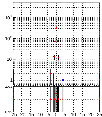
N of associated tracks (simToReco) vs dxy(PV)
