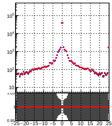
—■— DQM_TT_mkFit-DQM_lowptq_orig —●— DQM_TT_mkFit-DQM_lowptq_modi2
