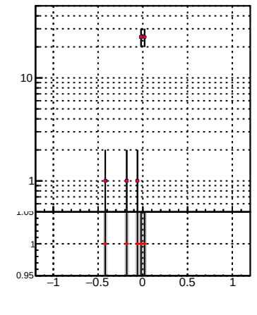
N of associated tracks (simToReco) vs dz(PV) zoomed
