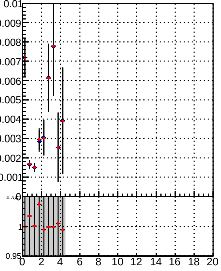
Fake rate vs. — \bullet DQM TT mkFit-DQM_lowptq_orig — \bullet DQM TT mkFit-DQM_lowptq_modi2
