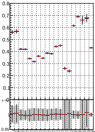
Fake rate vs. — \bullet DQM TT mkFit-DQM_lowptq_orig — \bullet DQM TT mkFit-DQM_lowptq_modi2
