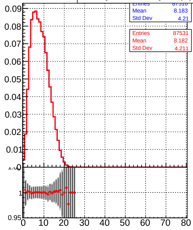
Legend: DQM_TT_mkFit-DQM_lowptq_orig (grey bars), DQM_TT_mkFit-DQM_lowptq_modi2 (red line with dots)
