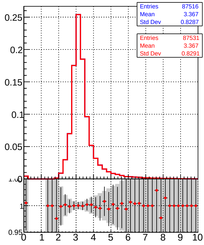
Legend: DQM_TT_mkFit-DQM_lowptq_orig (grey bars), DQM_TT_mkFit-DQM_lowptq_modi2 (red line with dots)
