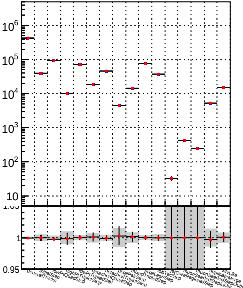
Number —●— DQM_TT_mkFit-DQM_lowptq_mc
