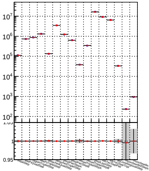
Number —●— DQM_TT__mkFit-DQM_lowptq_modi2
