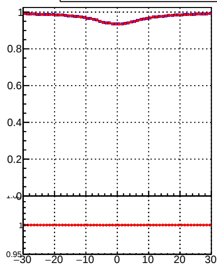
—•— DQM_TT_mkFit-DQM_lowptq_orig —•— DQM_TT_mkFit-DQM_lowptq_mod2
