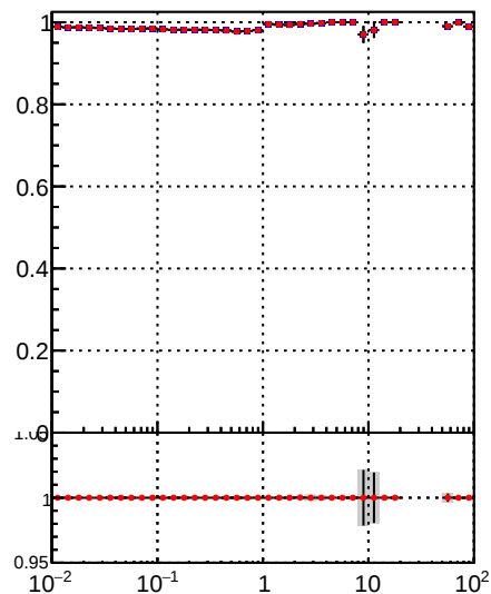
—•— DQM_TT_mkFit-DQM_lowptq_orig —•— DQM_TT_mkFit-DQM_lowptq_mod2
