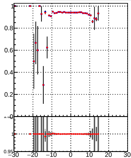
—•— DQM_TT_mkFit-DQM_lowptq_orig —•— DQM_TT_mkFit-DQM_lowptq_modi2
