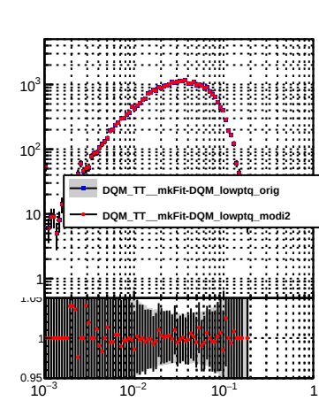
N of reconstructed tracks vs dR(track,jet)
