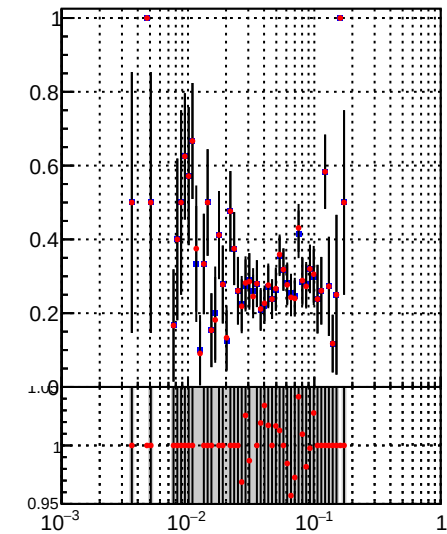
—•— DQM_TT_mkFit-DQM_lowptq_orig —•— DQM_TT_mkFit-DQM_lowptq_modi2
