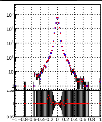
Fit-DQM_lowptq_modi2
