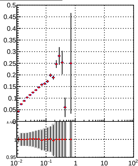
—•— DQM_TT_mkFit-DQM_lowptq_orig —•— DQM_TT_mkFit-DQM_lowptq_modi2
