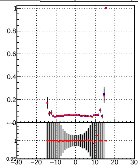
—•— DQM_TT_mkFit-DQM_lowptq_orig —•— DQM_TT_mkFit-DQM_lowptq_modi2
