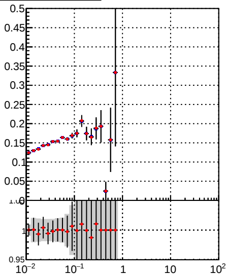
—•— DQM_TT_mkFit-DQM_lowptq_orig —•— DQM_TT_mkFit-DQM_lowptq_modi2
