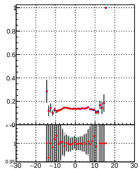
Fake rate vs d —•— DQM TT mkFit-DQM_lowptq_orig —•— DQM TT mkFit-DQM_lowptq_mod12
