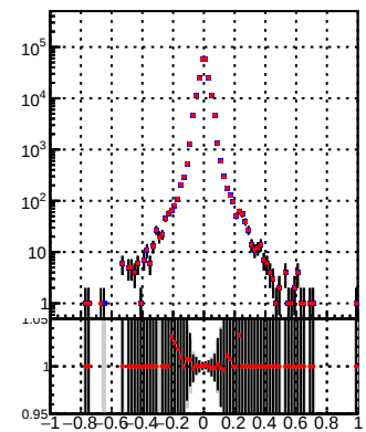
Legend: DQM_TT_mkFit-DQM_lowptq_orig (black line) DQM_TT_mkFit-DQM_lowptq_modi2 (red line)
