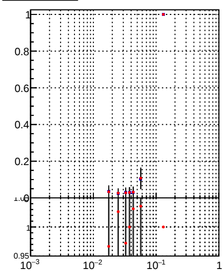
Fake rate vs dr Legend: DQM_TT_mkFit-DQM_lowptq_orig DQM_TT_mkFit-DQM_lowptq_modi2
