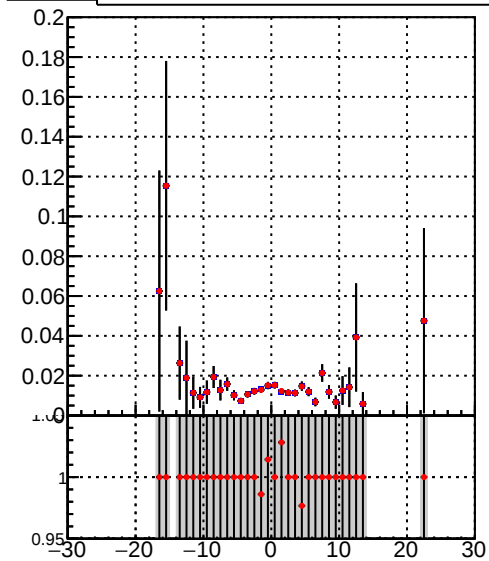
Efficiency vs vertpos — DQM_TT_mkFit-DQM_lowptq_orig — DQM_TT_mkFit-DQM_lowptq_modi2
