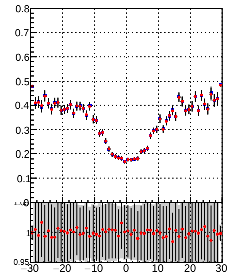
—●— DQM_TT_mkFit-DQM_lowptq_orig —●— DQM_TT_mkFit-DQM_lowptq_mod12
