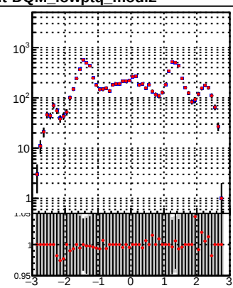
—•— DQM_TT_mkFit-DQM_lowptq_orig —•— DQM_TT_mkFit-DQM_lowptq_modi2
