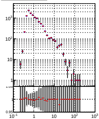
—•— DQM_TT_mkFit-DQM_lowptq_orig —•— DQM_TT_mkFit-DQM_lowptq_modi2
