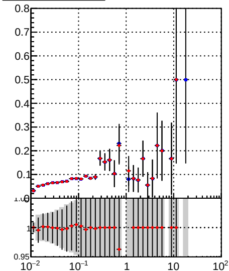
—•— DQM_TT_mkFit-DQM_lowptq_orig —•— DQM_TT_mkFit-DQM_lowptq_modi2
