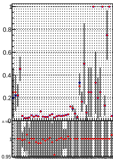
Fake rate vs. —•— DQM TT mkFit-DQM_lowptq_orig —•— DQM TT mkFit-DQM_lowptq_modi2
