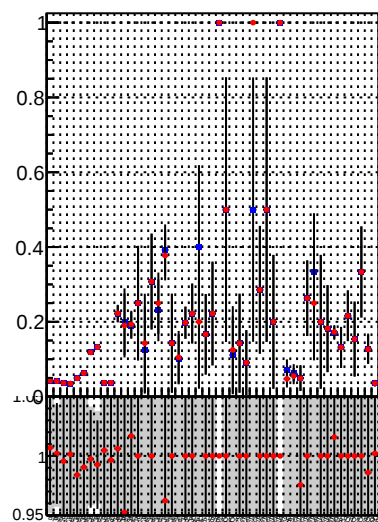
Fake rate vs. DQM TT mkFit-DQM_lowptq_orig DQM TT mkFit-DQM_lowptq_mod12
