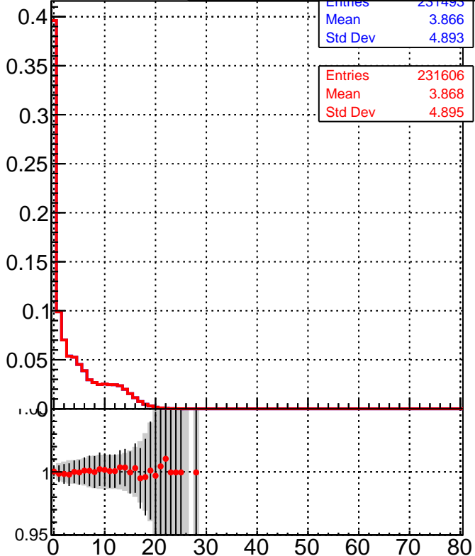
■ DQM_TT_mkFit-DQM_lowptq_orig ● DQM_TT_mkFit-DQM_lowptq_modi2
