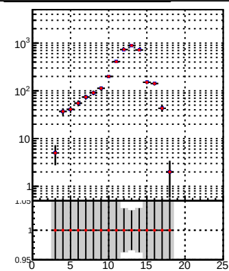
—•— DQM_TT_mkFit-DQM_lowptq_orig —•— DQM_TT_mkFit-DQM_lowptq_modi2
