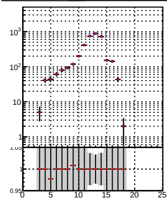
—•— DQM_TT_mkFit-DQM_lowptq_orig —•— DQM_TT_mkFit-DQM_lowptq_modi2
