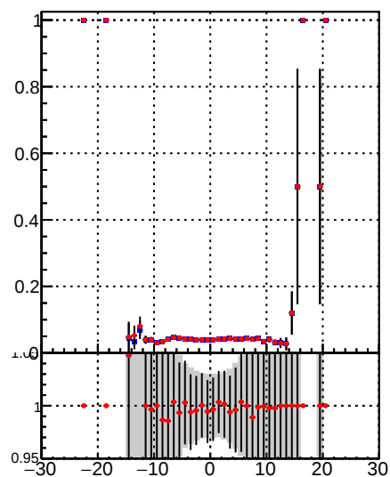
—•— DQM_TT_mkFit-DQM_lowptq_orig —•— DQM_TT_mkFit-DQM_lowptq_modI2
