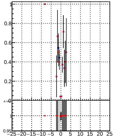
—•— DQM_TT_mkFit-DQM_lowptq_orig —•— DQM_TT_mkFit-DQM_lowptq_modI2
