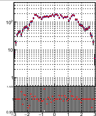
it-DQM_lowptq_orig it-DQM_lowptq_modi2
