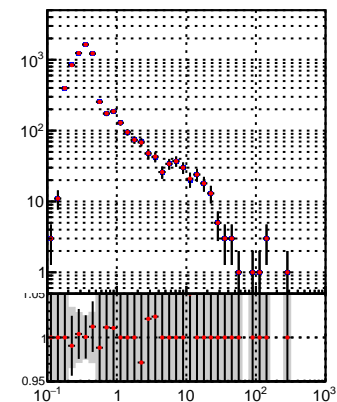
it-DQM_lowptq_orig it-DQM_lowptq_modi2
