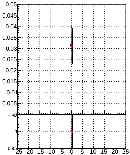
Fake rate vs d —•— DQM TT mkFit-DQM_lowptq_orig —•— DQM TT mkFit-DQM_lowptq_mod12
