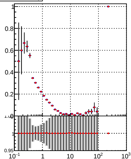
■ DQM_TT_mkFit-DQM_lowptq_orig ● DQM_TT_mkFit-DQM_lowptq_modi2
