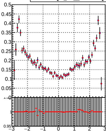
■ DQM_TT_mkFit-DQM_lowptq_orig ● DQM_TT_mkFit-DQM_lowptq_modi2
