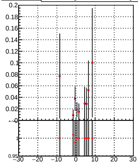
Fake rate vs verpos Legend: DQM_TT_mkFit-DQM_lowptq_orig DQM_TT_mkFit-DQM_lowptq_modi2
