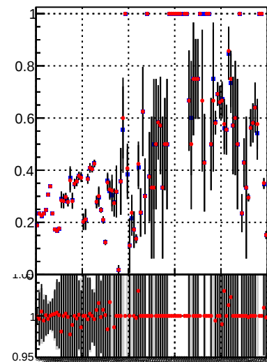
Fake rate vs. — DQM TT mkFit-DQM_lowptq_orig — DQM TT mkFit-DQM_lowptq_modi2
