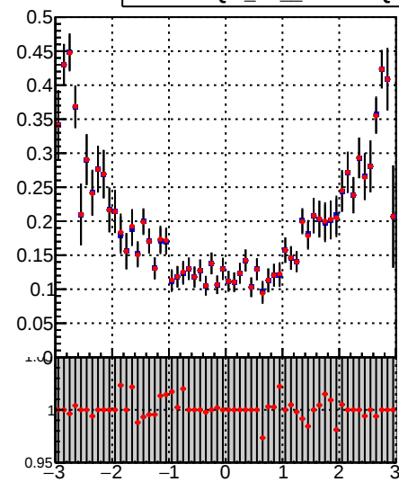
—•— DQM_TT_mkFit-DQM_lowptq_orig —•— DQM_TT_mkFit-DQM_lowptq_mod2
