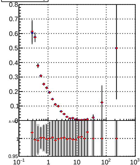
—•— DQM_TT_mkFit-DQM_lowptq_orig —•— DQM_TT_mkFit-DQM_lowptq_mod2
