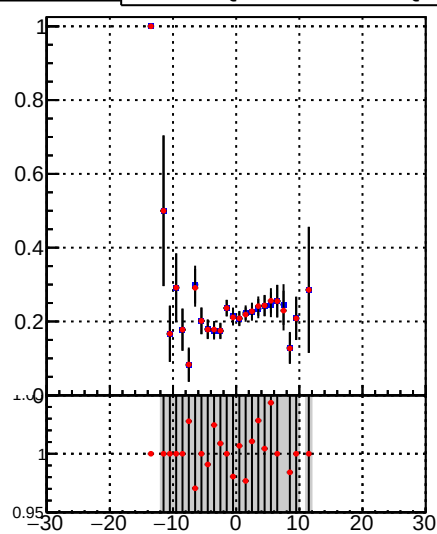
—•— DQM_TT_mkFit-DQM_lowptq_orig —•— DQM_TT_mkFit-DQM_lowptq_modi2
