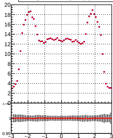
mean hit — DQM_TT_mkFit-DQM_lowptq_orig — DQM_TT_mkFit-DQM_lowptq_modi2
