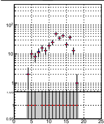
N of reco track vs hit DQM_TT_mkFit-DQM_lowptq_orig DQM_TT_mkFit-DQM_lowptq_modi2
