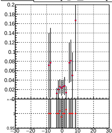
Fake rate vs v Legend: DQM_TT_mkFit-DQM_lowptq_orig (blue line with dots) DQM_TT_mkFit-DQM_lowptq_modi2 (red line with dots)
