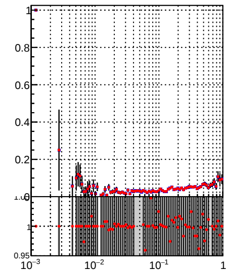
Fake rate vs dr DQM_TT_mkFit-DQM_lowptq_orig DQM_TT_mkFit-DQM_lowptq_modi2
