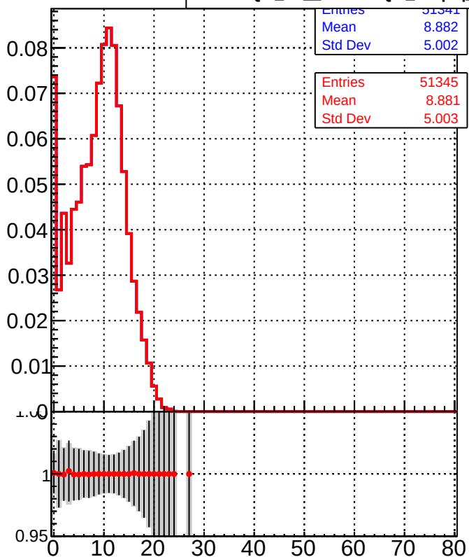
— DQM_TT_mkFit-DQM_lowptq_orig — DQM_TT_mkFit-DQM_lowptq_modi2
