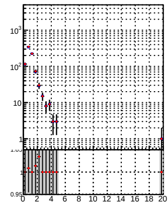
N of reco track vs. \chi^2 — mkFit-DQM_lowptq_orig — mkFit-DQM_lowptq_mod1 — mkFit-DQM_lowptq_mod2
