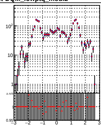
—●— DQM_TT_mkFit-DQM_lowptq_orig —●— DQM_TT_mkFit-DQM_lowptq_modi2
