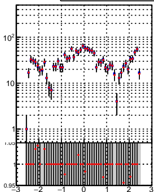
—•— DQM_TT_mkFit-DQM_lowptq_orig —•— DQM_TT_mkFit-DQM_lowptq_modi2
