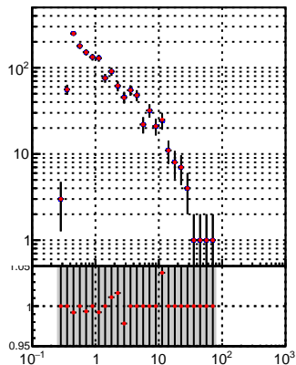
—•— DQM_TT_mkFit-DQM_lowptq_orig —•— DQM_TT_mkFit-DQM_lowptq_modi2
